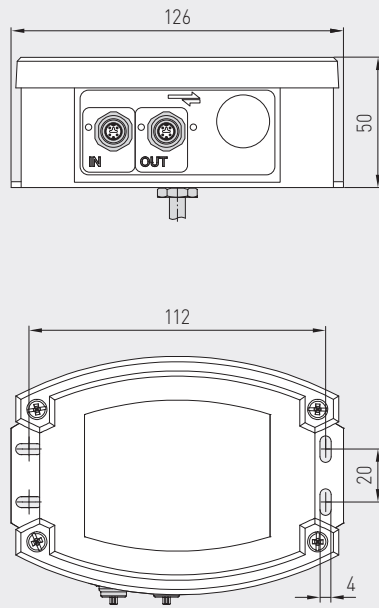
Dimensional drawing
