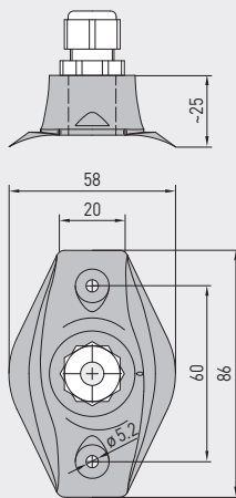
Dimensional drawing
