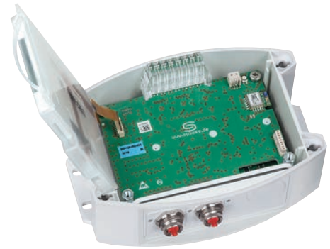
MWTM-EtherCAT P with display and bar graph
