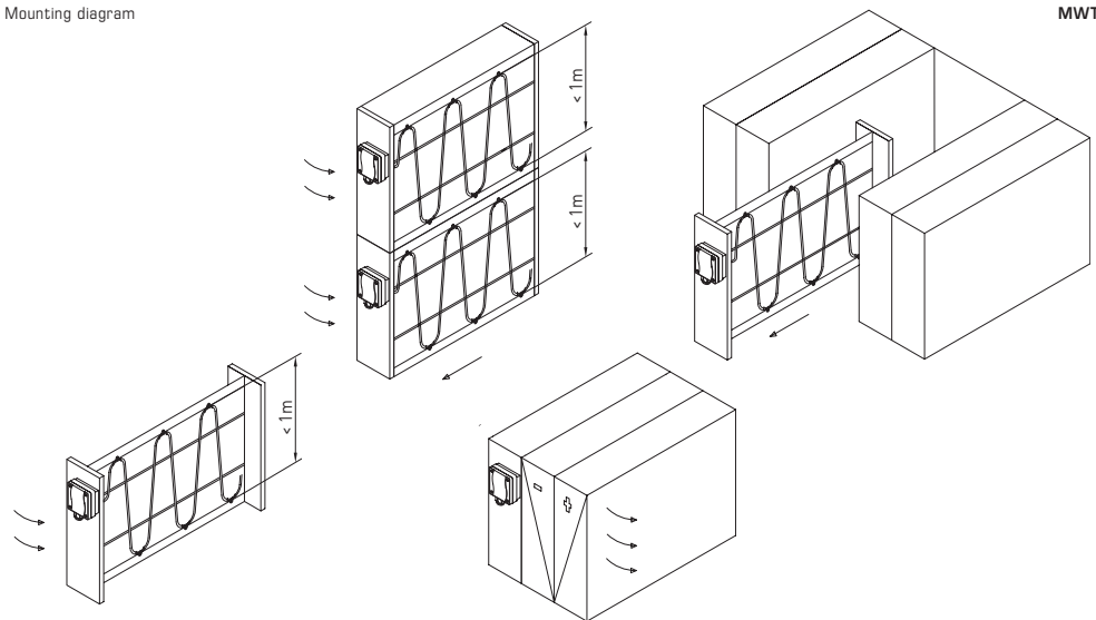
Mounting diagram
